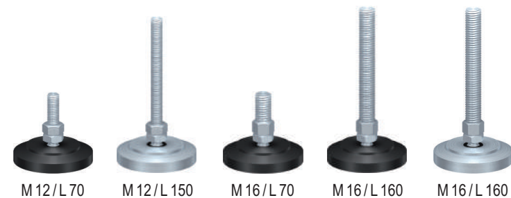
Adjustable Feet Ø79
