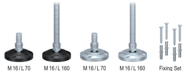
Fixing Set
