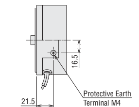
Detail Drawing of Protective Earth Terminal
